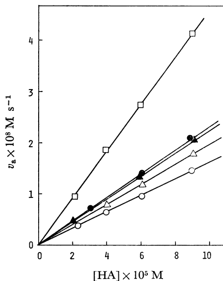
Fig. 3. Reaction of PNPA with a series of hydroxamic acids. ○: PHA-AAm-1, ● PHA-AAm-2; □ 2, ▲ 3, △ 4 pH=8.57, 30 °C, 1.4 vol% CH 3 CN-H 2 O, 0.1 M KCl, 0.05 M Tris., [PNPA]= 5.01 \times 10^{-5} M
