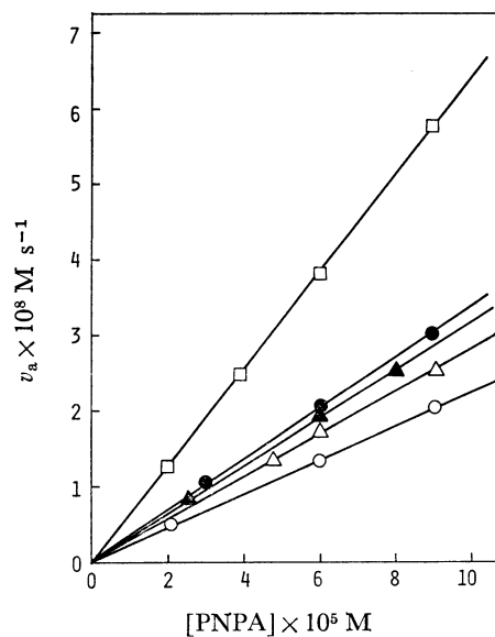
Fig. 4. Reaction of PNPA with a series of hydroxamic acids. ○ PHA-AAm-1, ● PHA-AAm-2, □ 2, ▲ 3, △ 4 pH=8.57, 30 °C, 1.4 vol% CH 3 CN-H 2 O, 0.1 M KCl, 0.05 M Tris., [HA]= 7.01 \times 10^{-5} M
